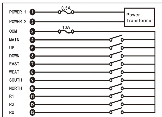
Q800 Wiring Diagram
