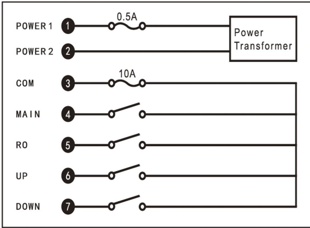
Q200 Wiring Diagram
