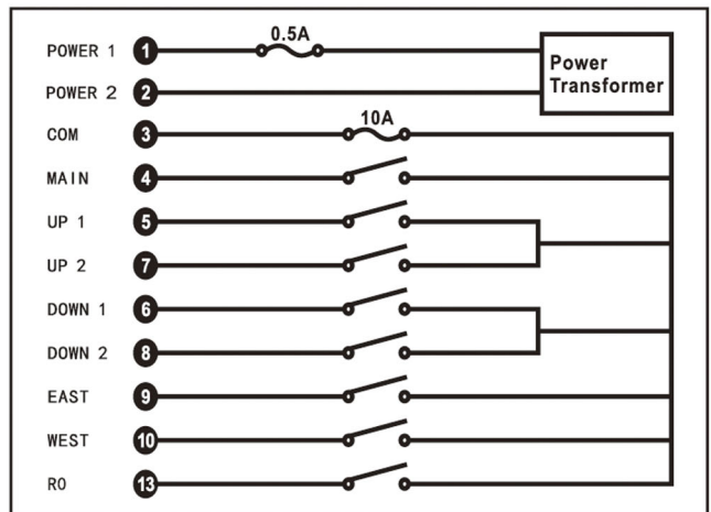
Q402 Wiring Diagram
