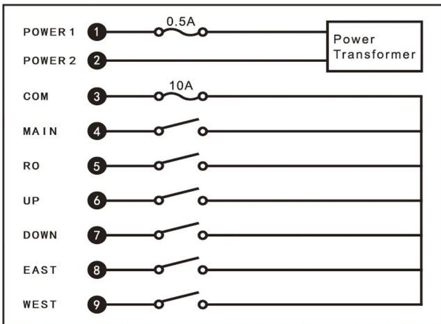
Q400 Wiring Diagram
