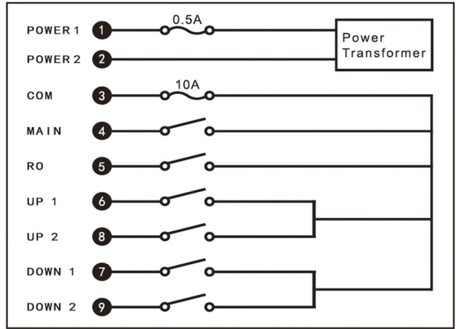
Q202 Wiring Diagram
